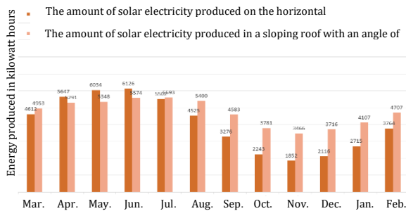
Figure 2. The solar electricity production was evaluated for both horizontal and sloping roofs with an angle of 35 degrees in the BAPV system.
