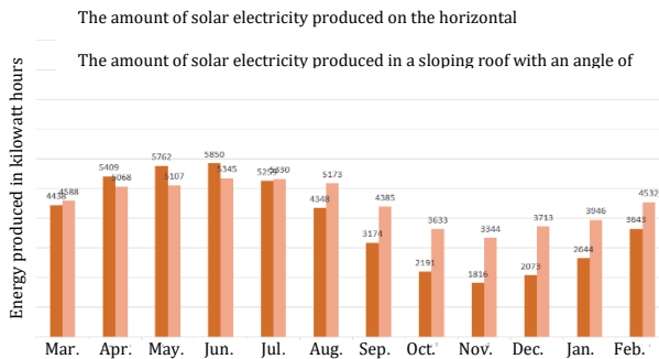
Figure 3. The amount of solar electricity produced in a horizontal roof and in a sloping roof with an angle of 35 degrees in the BIPV system
