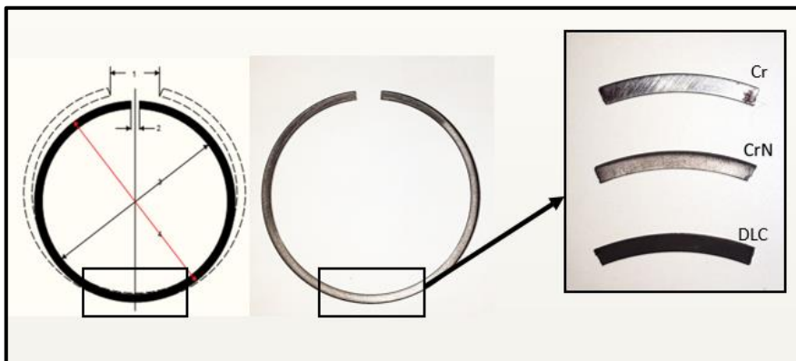
Figure 1. Piston ring wear sample after cutting
