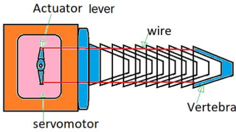
Figure 1. The WDFR components.
