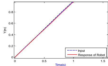
Figure 8. Convergence between WDFR response and ramp function as desired input.
