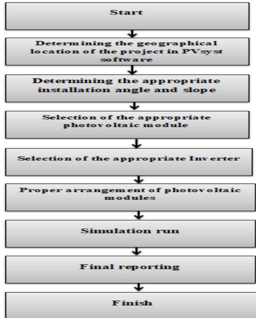
Figure 1. Design steps of the FTP panel.
